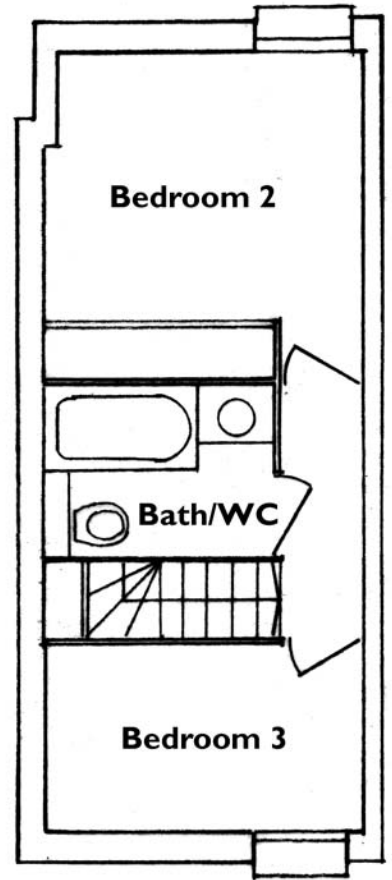
2nd Floor
