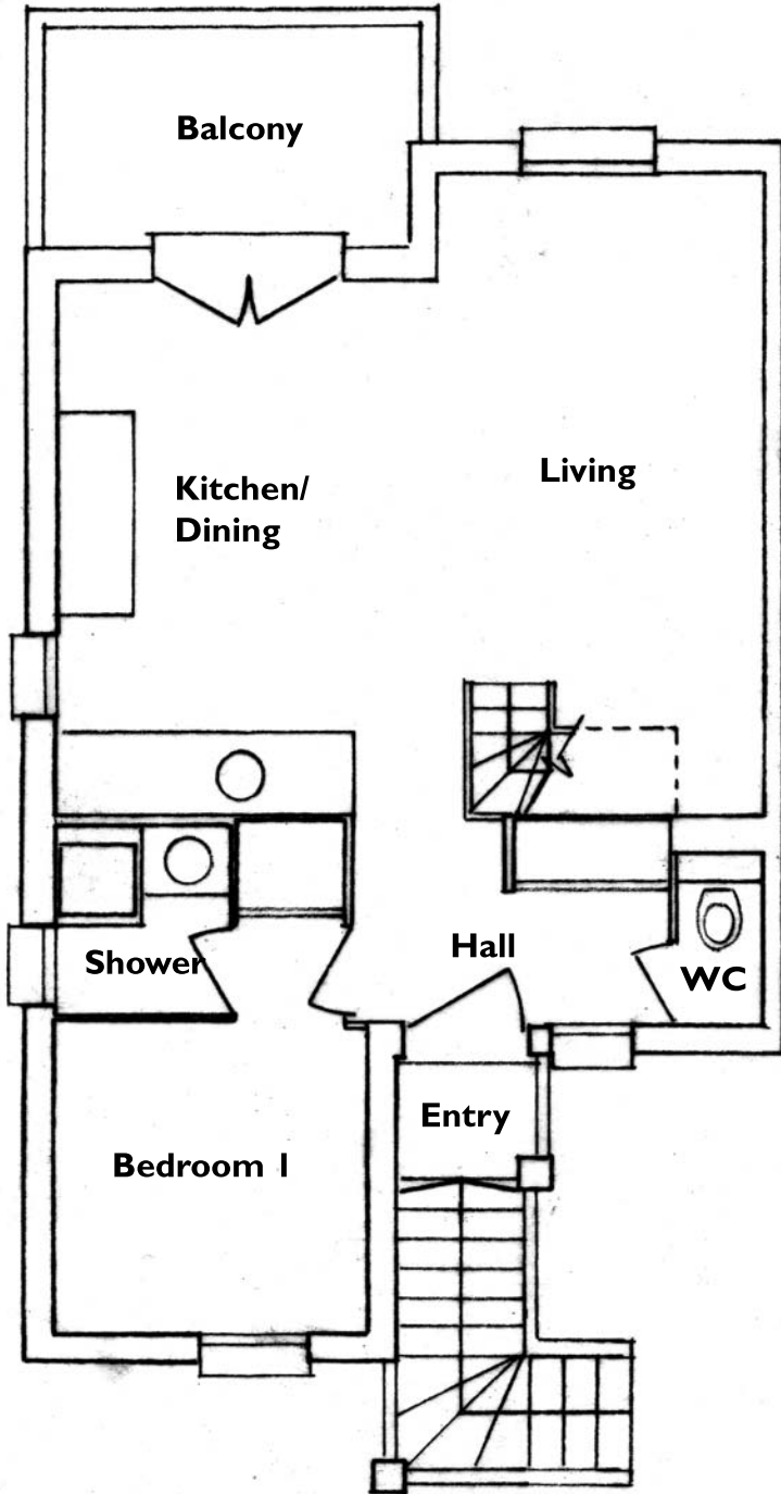
Chalet Joyvue 1st Floor
